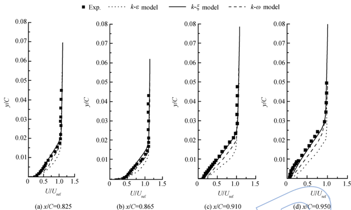
Fig. 2 Streamwise velocity profile at the location of AS240 at 8^\circ attack angle
