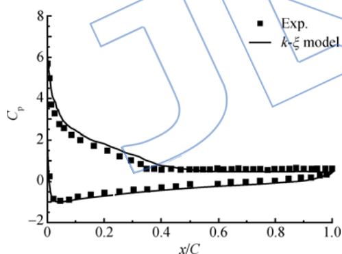
Fig. 3 Pressure coefficient of AS240 at 19^\circ attack angle
