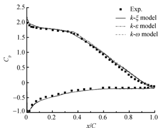
Fig. 1 Pressure coefficient of AS240 at 8^\circ attack angle
