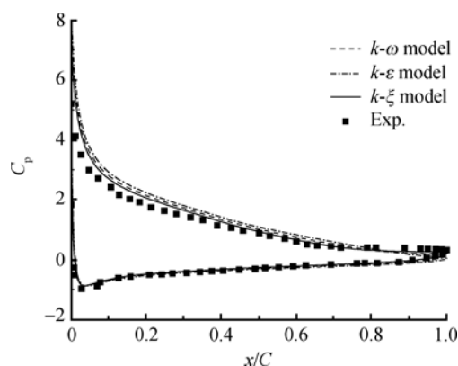
Fig. 4 Pressure coefficient of NACA4412 airfoil at 13.87^\circ attack angle
